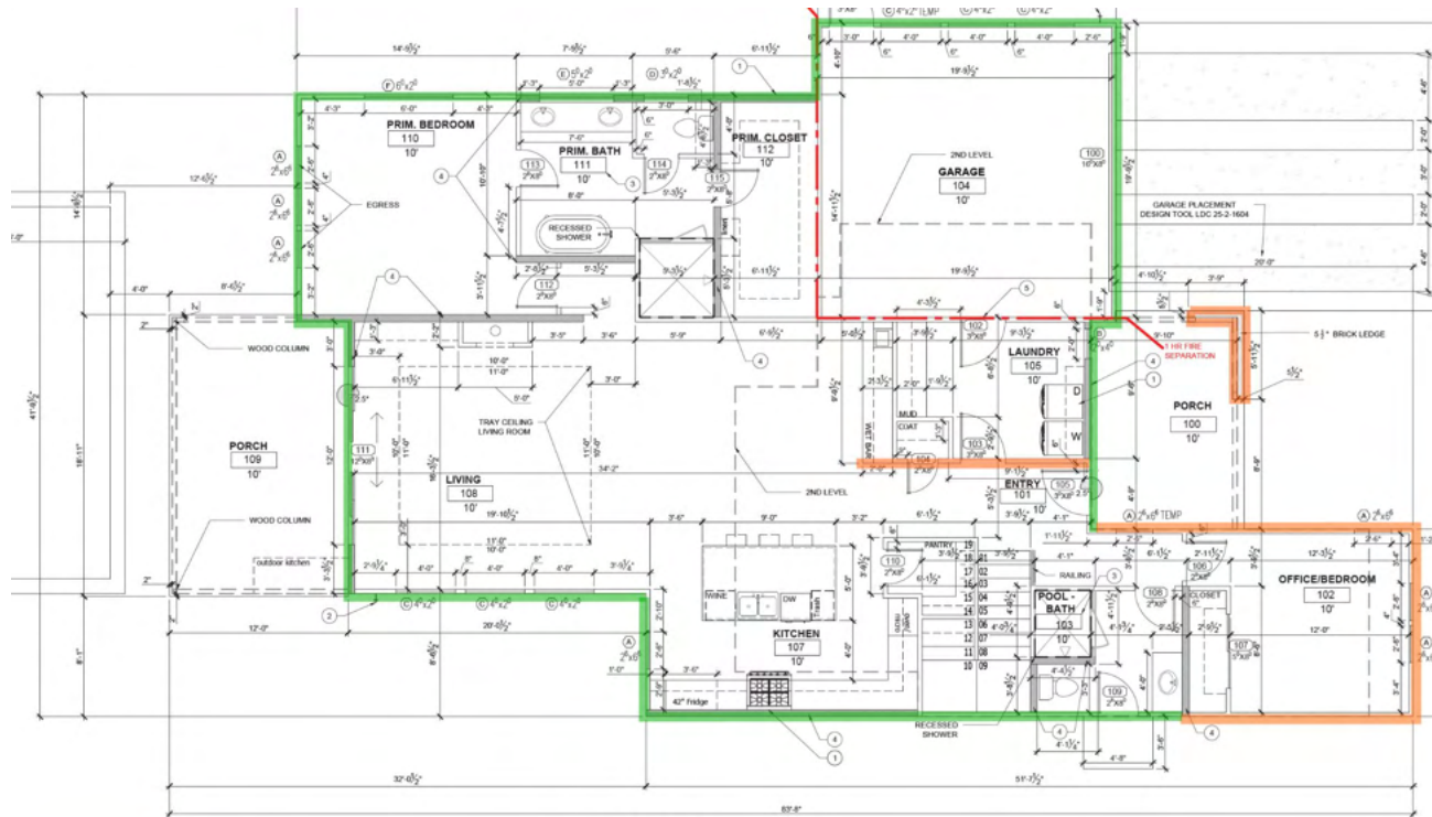
1 1ST FLOOR PLAN SCALE: 1/4"=1'-0"
